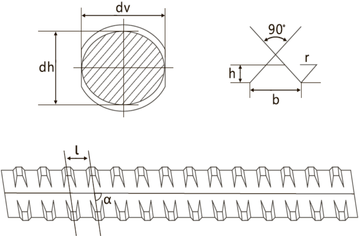
Yidao stress bar Hot rolled-Right hand thread
